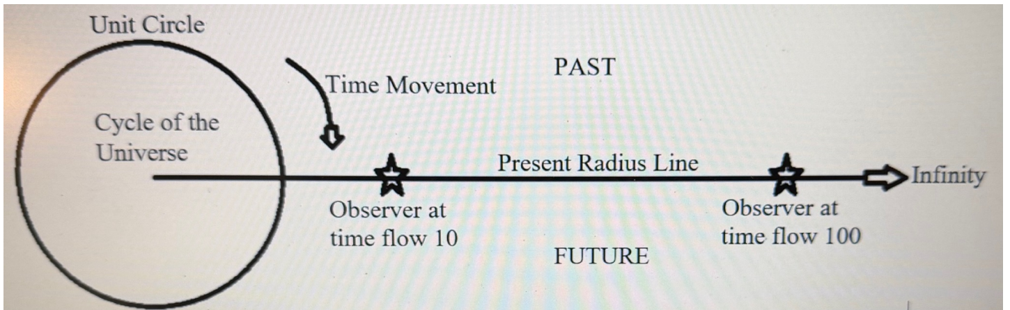
Figure 3.1: Unit Circle
