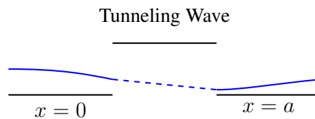
Figure 10.1: Visualization of electron spin wave tunneling through a rectangular barrier ( V = 1 eV or 2 eV, a = 1 nm).
