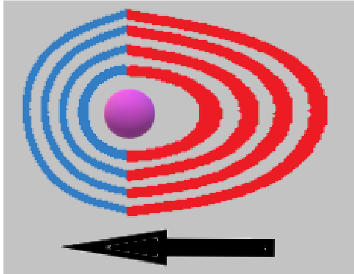
Figure 3: Spin wave compression in \xi M - Field
