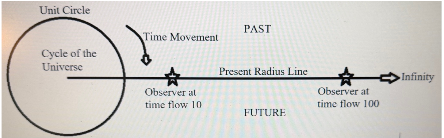
Figure 1: Unit Circle
